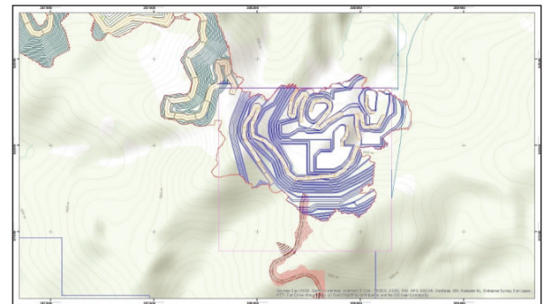
Desain Pit HL03
